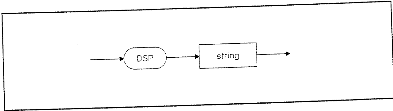
Figure 2-13. DSP Syntax Diagram
